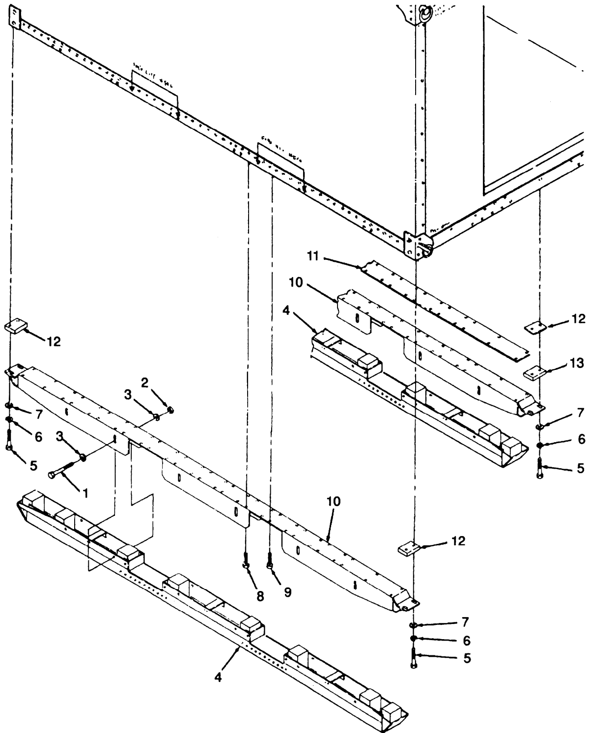
Figure 10. Skid Assembly and Mounting Brackets.
